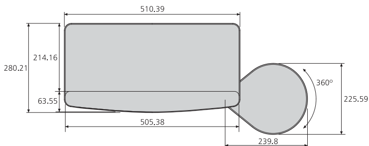
TRAY 201
