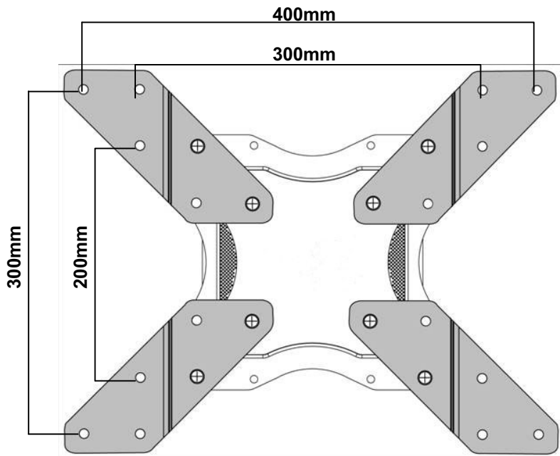
OPTION B for VESA hole patterns of: 200x300mm – 300x300mm – 300x400mm
