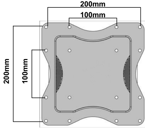
OPTION A for VESA hole patterns of: 100x100mm – 100x200mm - 200x100mm – 200x200mm
