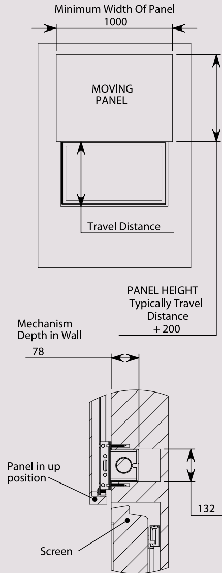
SECTION THROUGH MECHANISM
