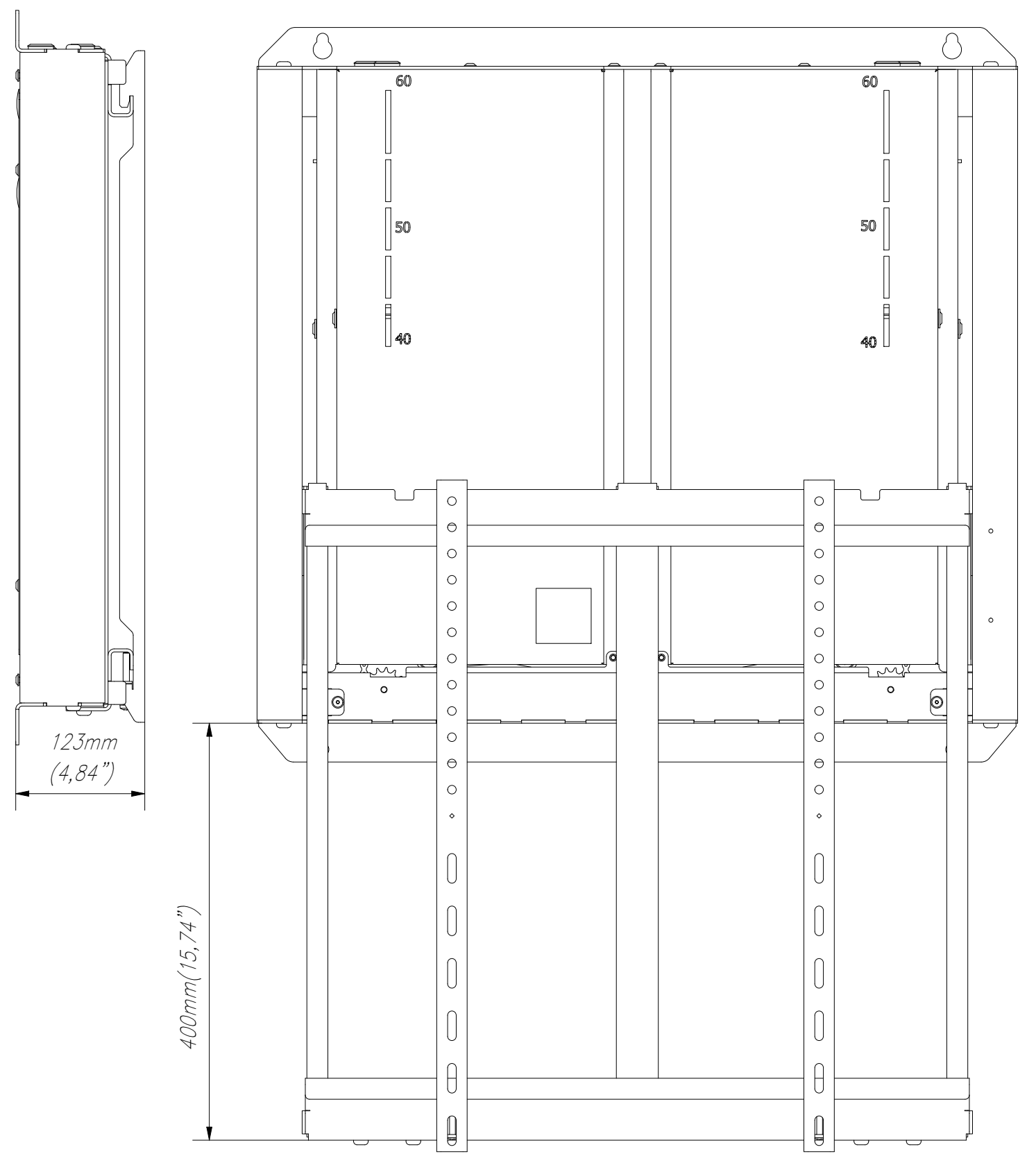
SIDE VIEW
