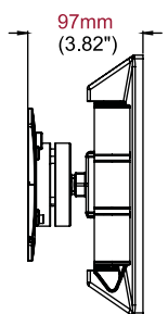
SIDE VIEW RETRACTED
