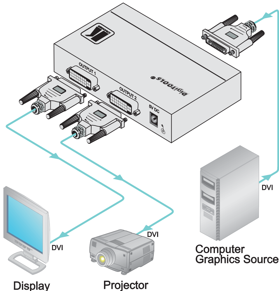
Figure 2: Connecting a VM-2HDCPx1 1:2 DVI Distributor
